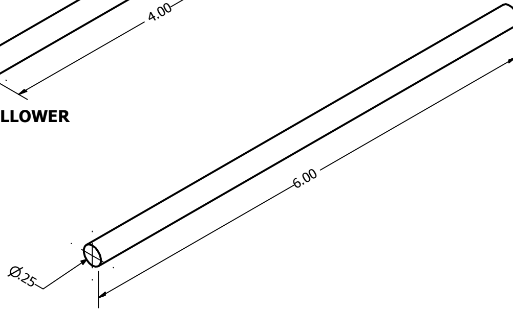
AXLE
